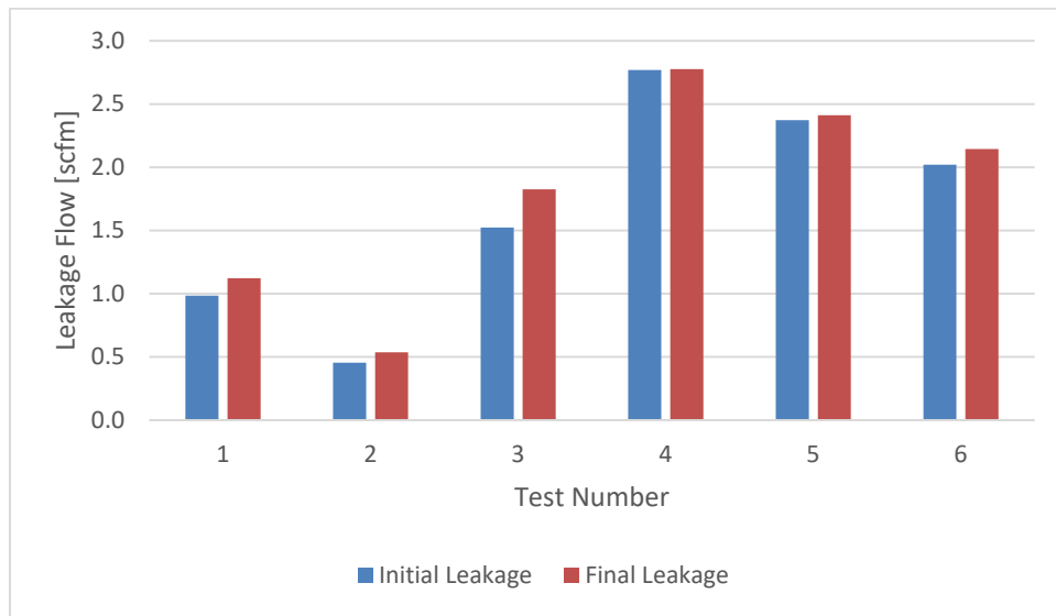
Figure 38. Change in Leakage After 1,000 Cycles of 800 Pa
